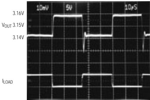
LOAD TRANSIENT
