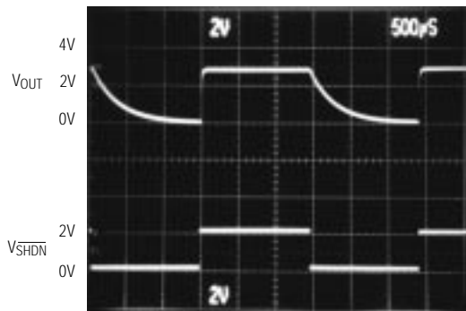
MAX8864 SHUTDOWN (NO LOAD)
