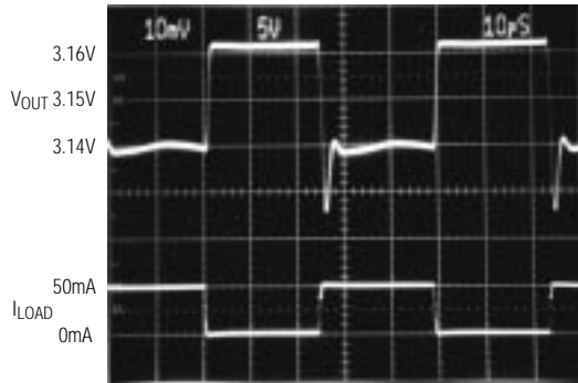
LOAD TRANSIENT
