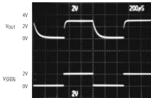
MAX8864 SHUTDOWN
